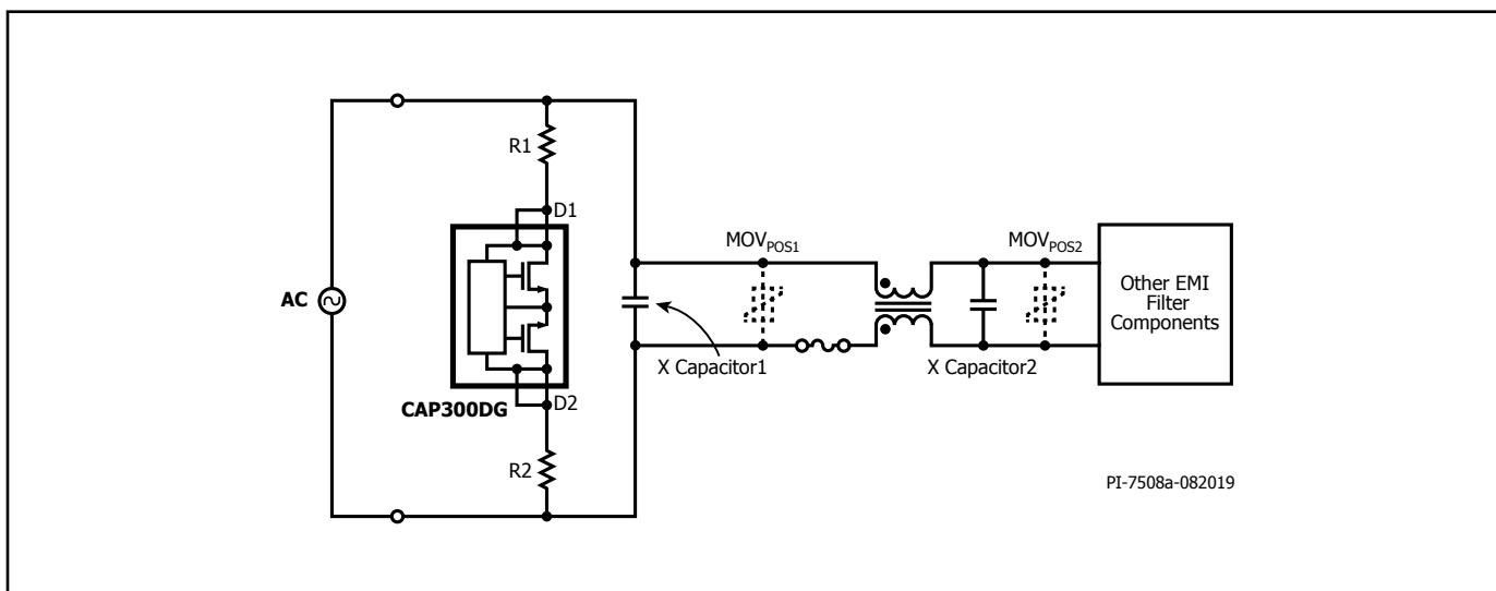
Figure 5. Placement Options of MOV.
