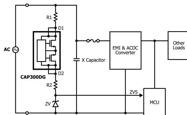
Figure 2. With Added Lossless ZC Output Signal (Non-Isolated System Example Shown). See DER-320 Design Report for Implementation Details of Other Configurations.
