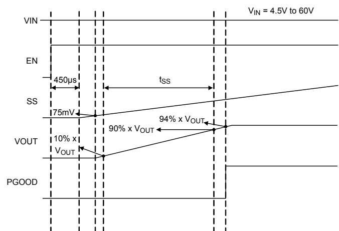
Figure 1 Start-Up Sequence for RTQ2962GQW
