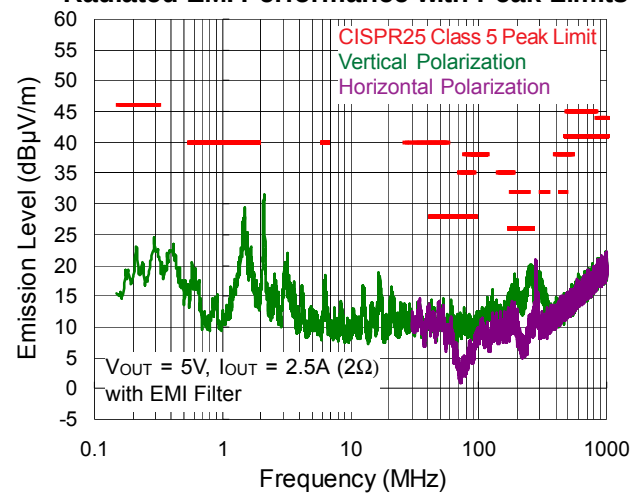
Radiated EMI Performance with Peak Limits
