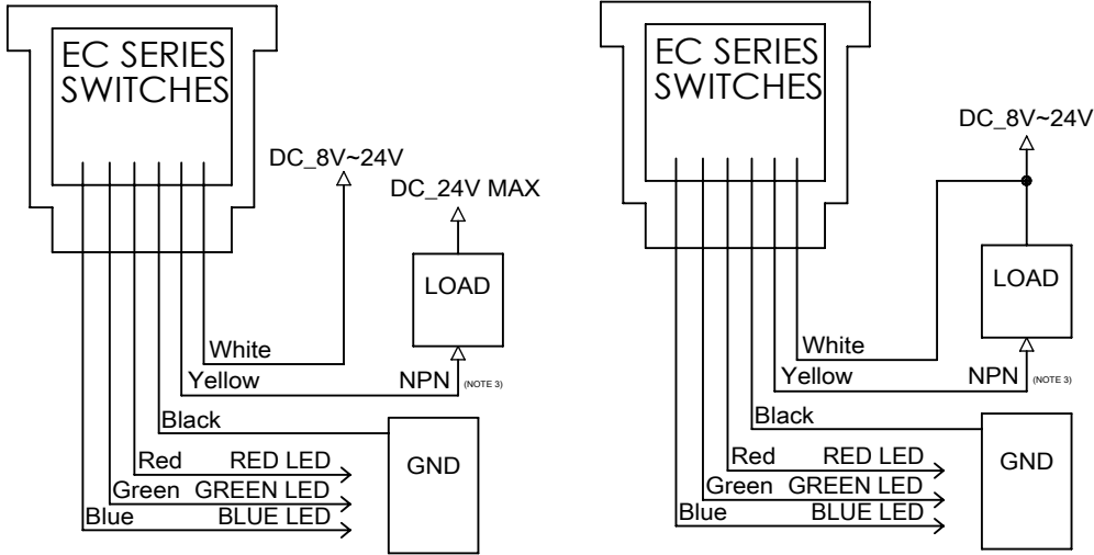
SUGGESTED CIRCUITRY
