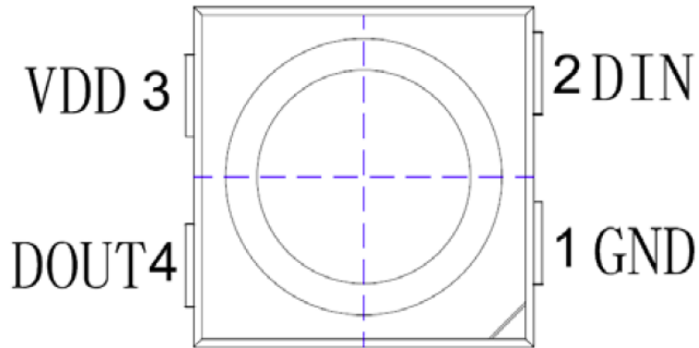
Figure 2. IN- PI33TBTPRGPB Pin Configuration
