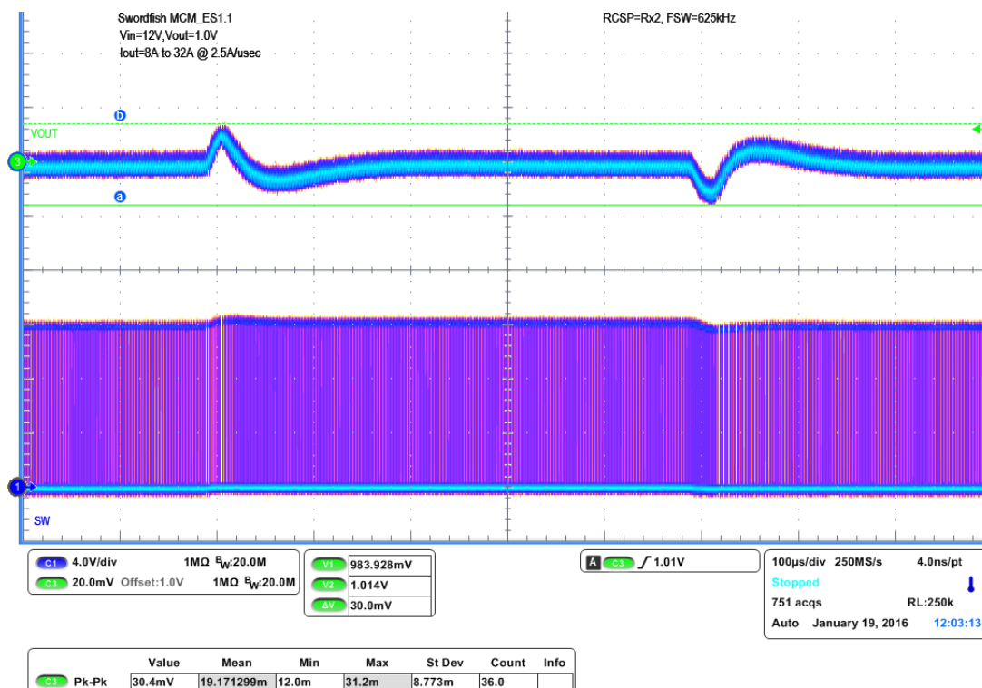
Figure 9-4. Transient Response of 1-V Output at 12 V_{IN} , Transient is 8 A to 32 A, 2.5 A/μs
