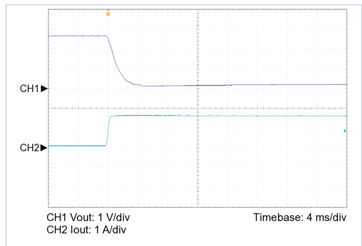
Figure 8 — 10% to 100% load transient response, V_{IN} = 42\text{ V} , nominal trim, C_{OUT\_EXT} = 200\text{ }\mu\text{F}
