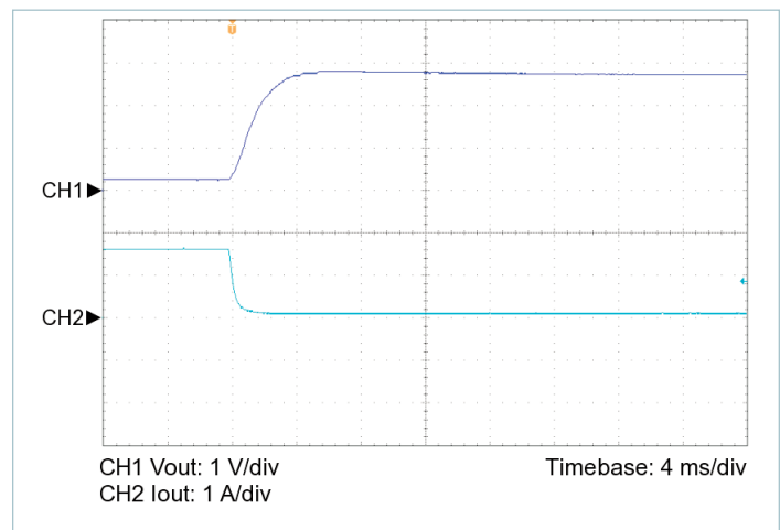
Figure 7 — 100% to 10% load transient response, V_{IN} = 42\text{ V} , nominal trim, C_{OUT\_EXT} = 200\text{ }\mu\text{F}
