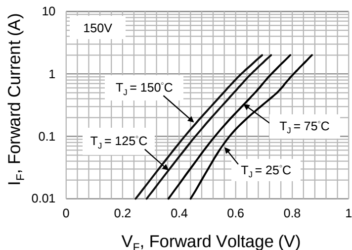
Fig.7 Typical Forward Characteristics
