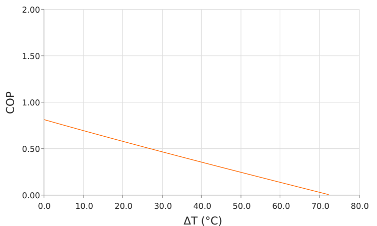
Coefficient of Performance (COP = Q_c/P_{in} ) T_{hot} = 27\text{ }^{\circ}\text{C} | Current = 6.1 Amps
