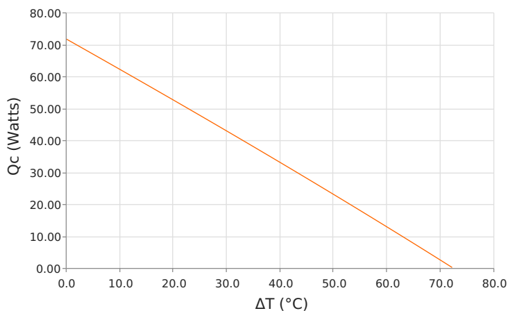
Heat Pumped at Cold Side ( Q_c ) T_{hot} = 27\text{ }^{\circ}\text{C} | Current = 6.1 Amps
