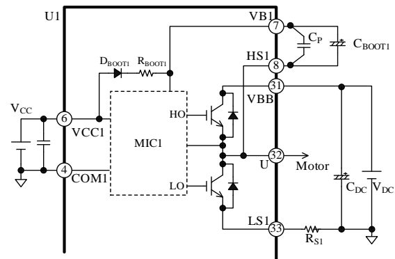
Figure 12-1. Bootstrap Circuit
