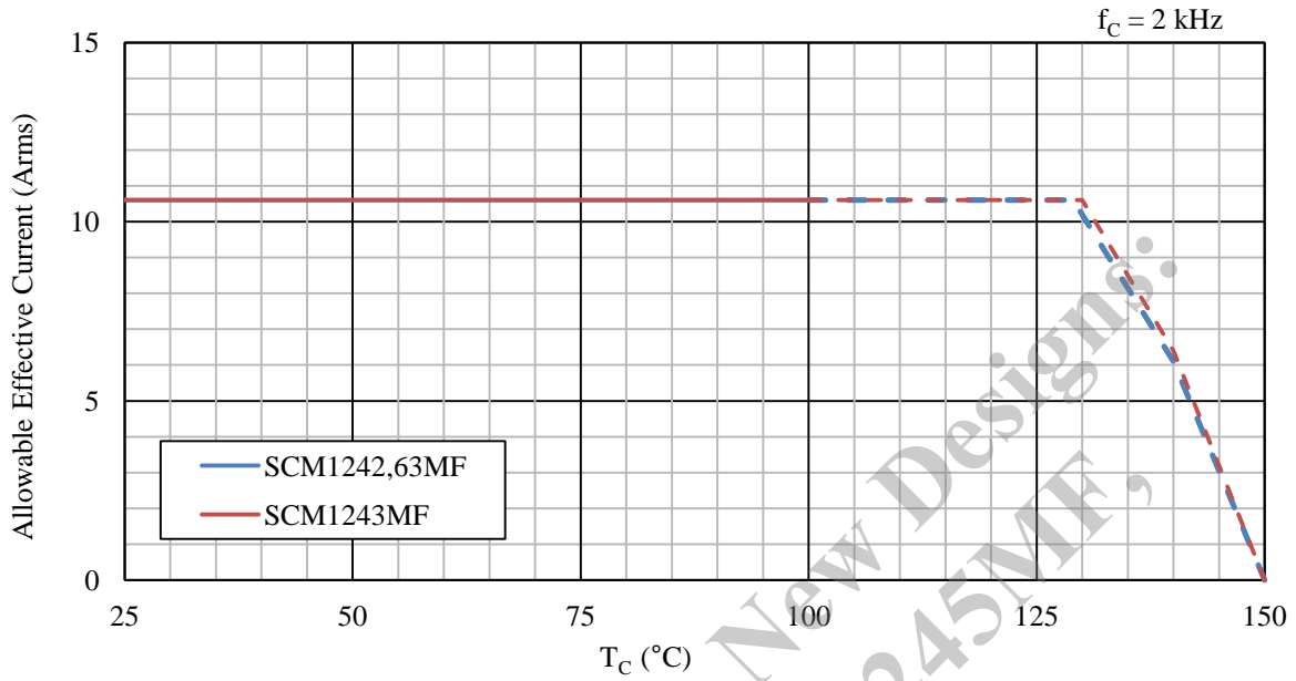
Figure 15-70. Allowable Effective Current ( f_C = 2 kHz): 15 A Devices
