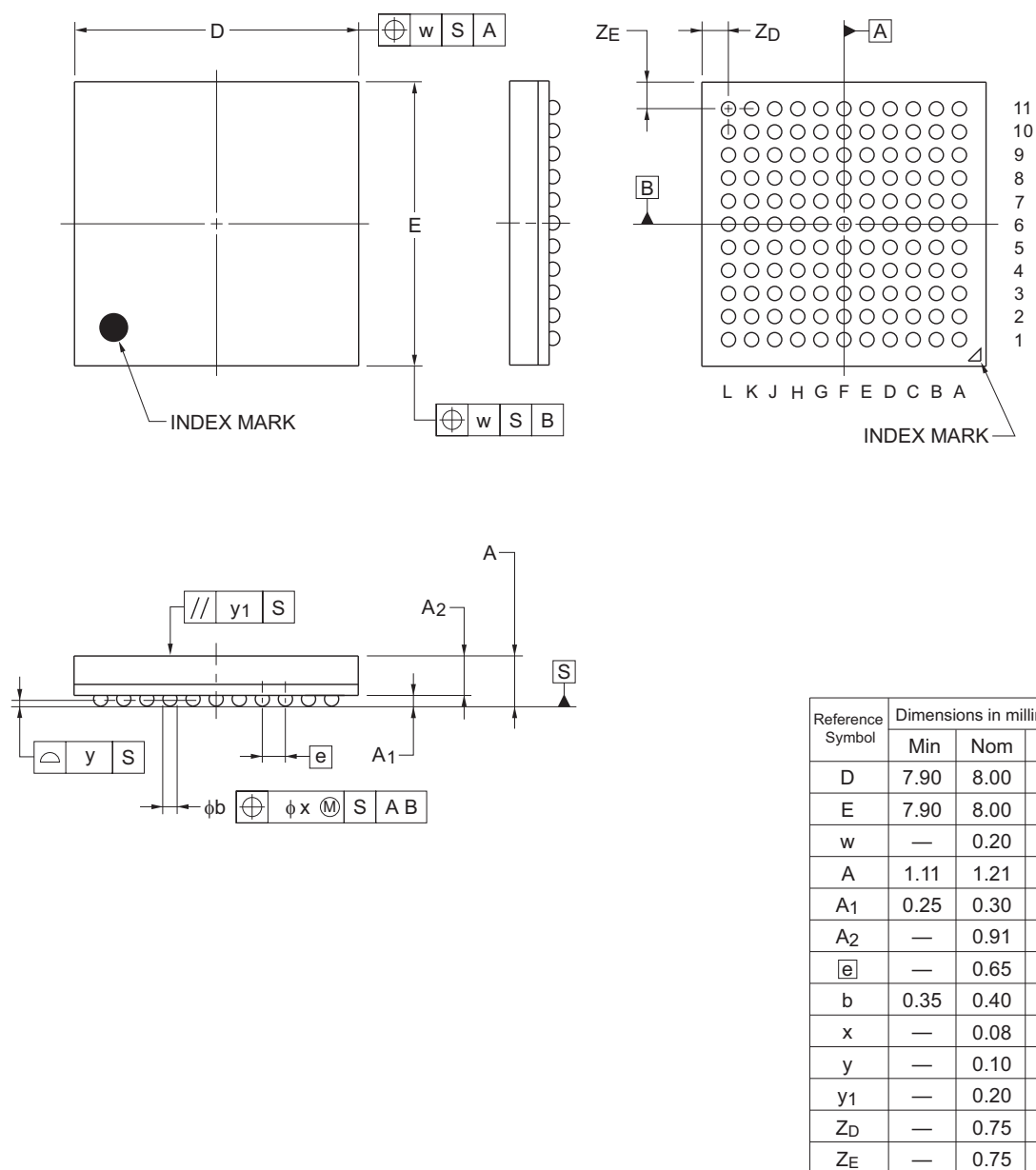
Figure 1.3 BGA 121-pin
