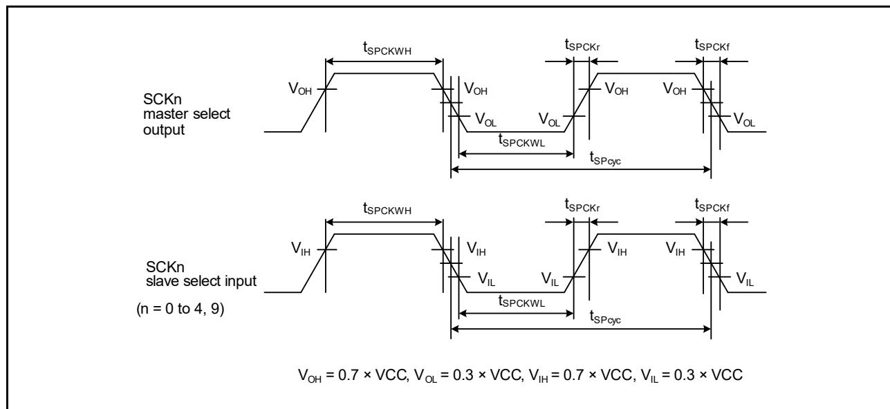
Figure 2.55 SCI simple SPI mode clock timing
