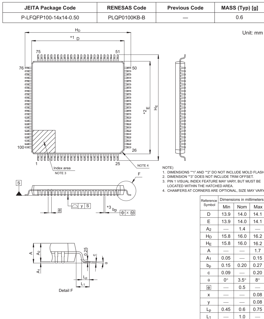
Figure 1.5 LQFP 100-pin
