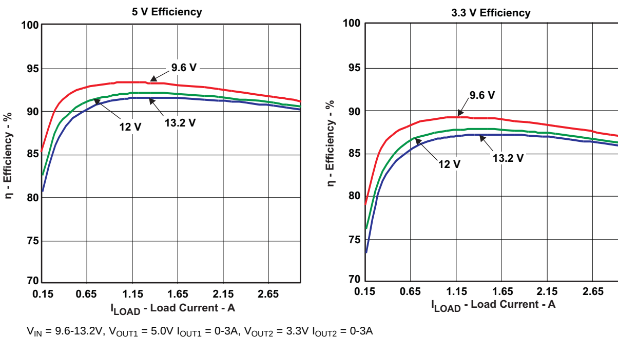
Figure 5. TPS55386EVM-363 Efficiency vs Load Current
