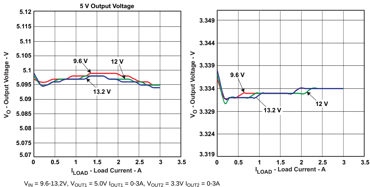
Figure 6. TPS55386EVM-363 Output Voltage vs Load Current
