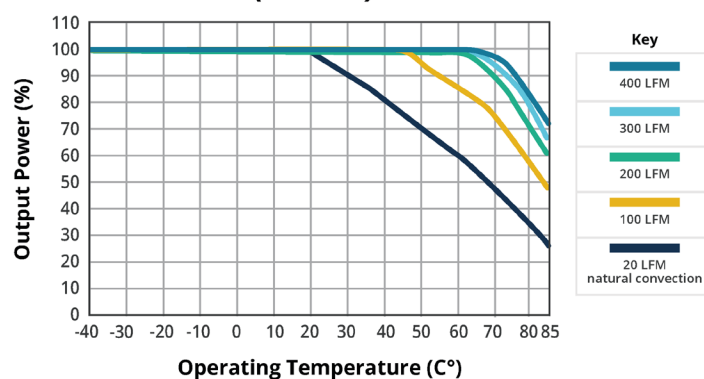
TEMPERATURE DERATING CURVE PRQ200W-Q48-S24-H-D (Heatsink version) ( V_{in} = 24\text{ V} )
