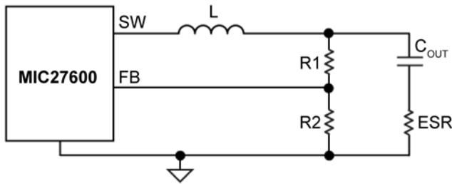
Figure 5a. Enough Ripple at FB
