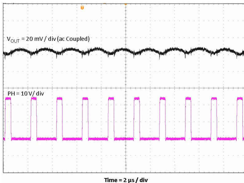
Figure 2-6. TPS54202EVM-716 Output Ripple, I_{OUT} = 2 A
