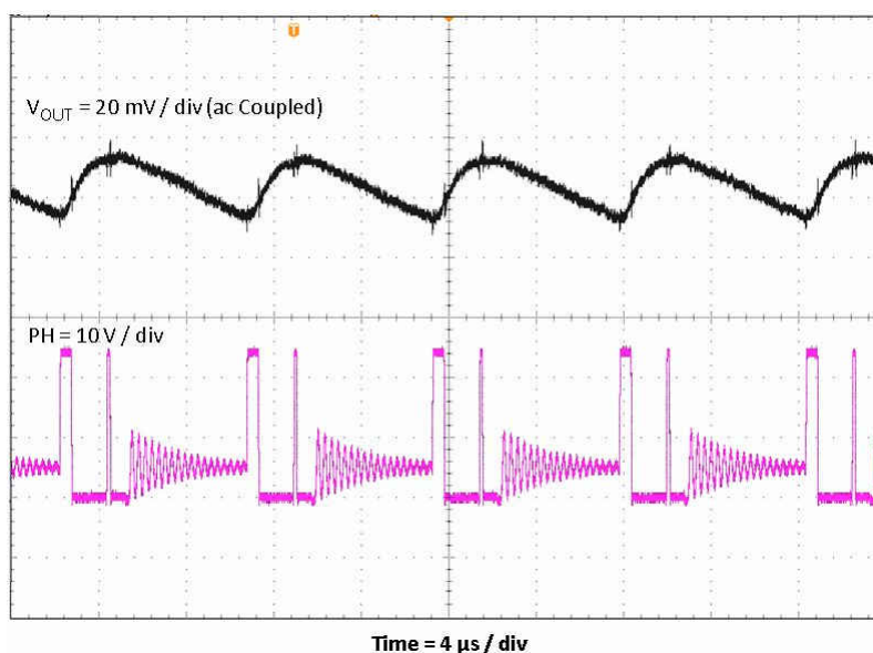
Figure 2-7. TPS54202EVM-716 Output Ripple, I_{OUT} = 100 mA
