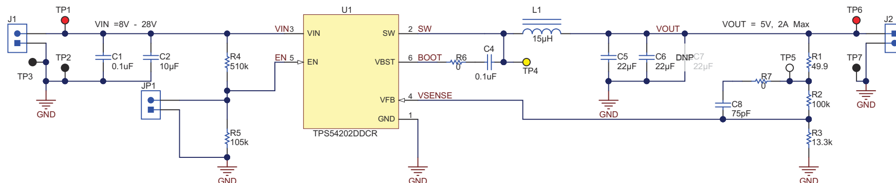
Figure 4-1. TPS54202EVM-716 Schematic
