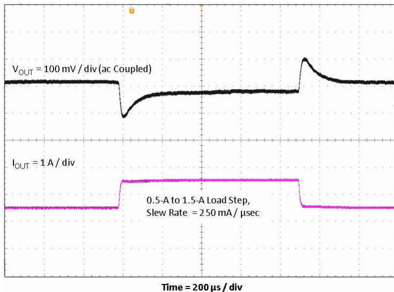
Figure 2-5. TPS54202EVM-716 Transient Response
