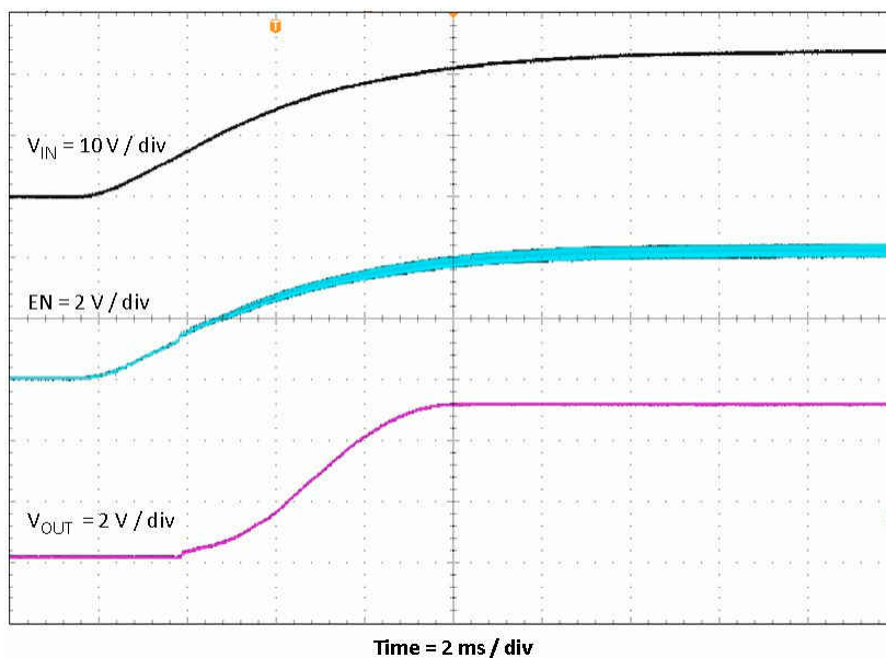
Figure 2-11. TPS54202EVM-716 Startup Relative to V_{IN}
