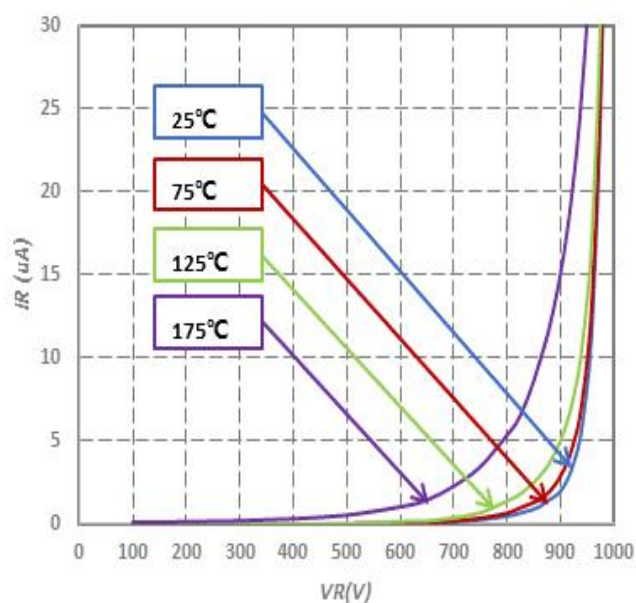
Fig.2-Typical Reverse Characteristics
