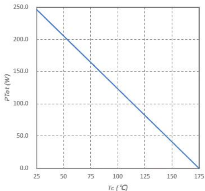
Fig.7-Power Derating
