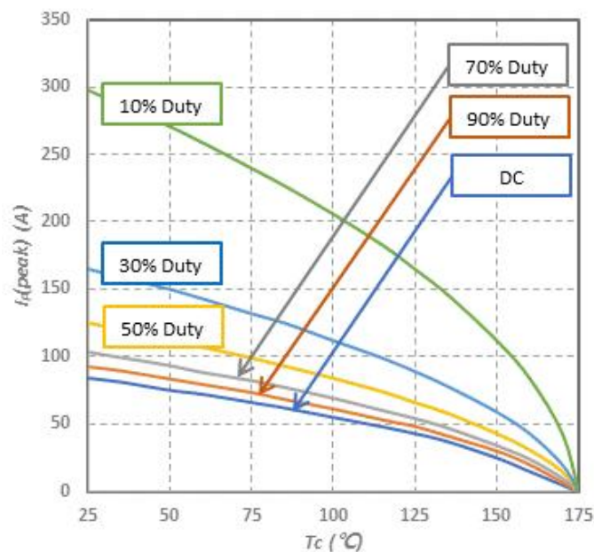
Fig.8-Current Derating
