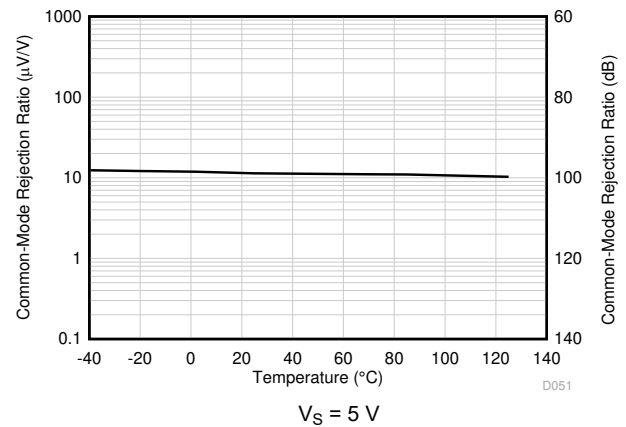
Figure 6-22. CMRR vs Temperature
