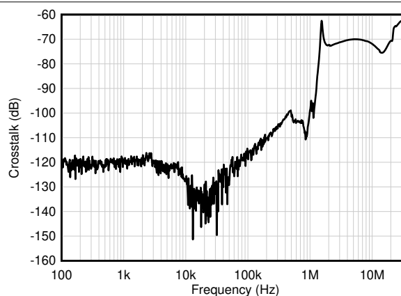
Figure 6-42. Channel Separation vs Frequency
