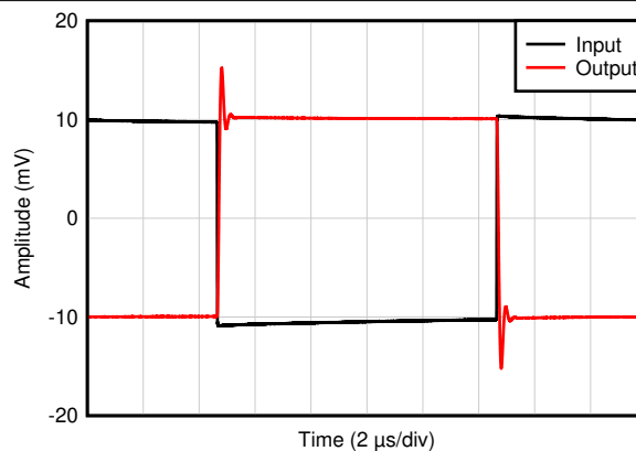
Figure 6-38. Small-Signal Step Response
