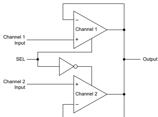
Figure 8-3. High Voltage Buffered Multiplexer
