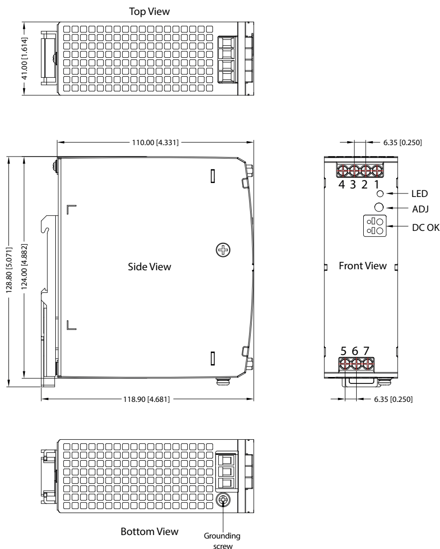
Figure 5. Mechanical Drawing
