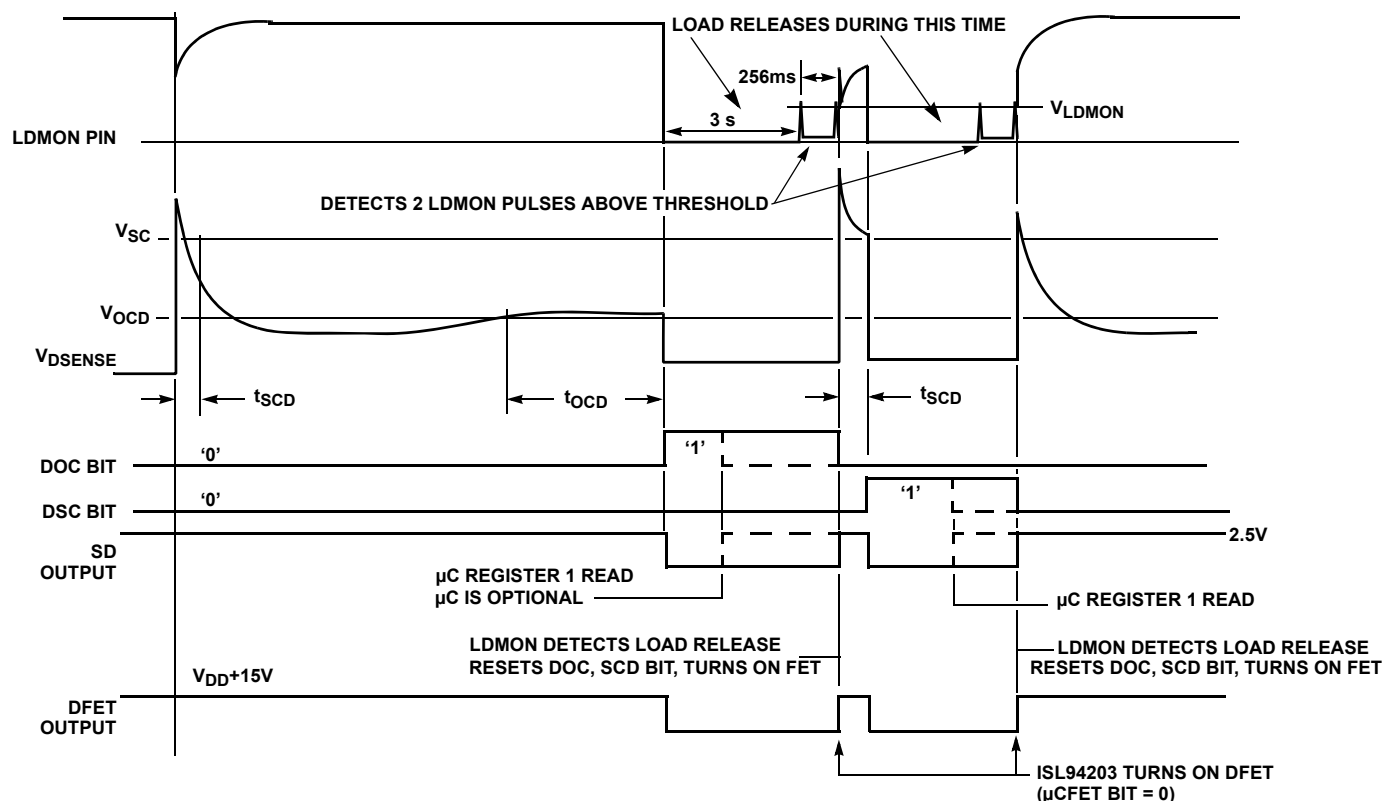
FIGURE 10. DISCHARGE/SHORT-CIRCUIT MONITOR
