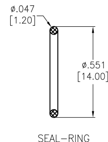
SEAL-RING
