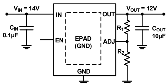
Figure 1. Typical Application
