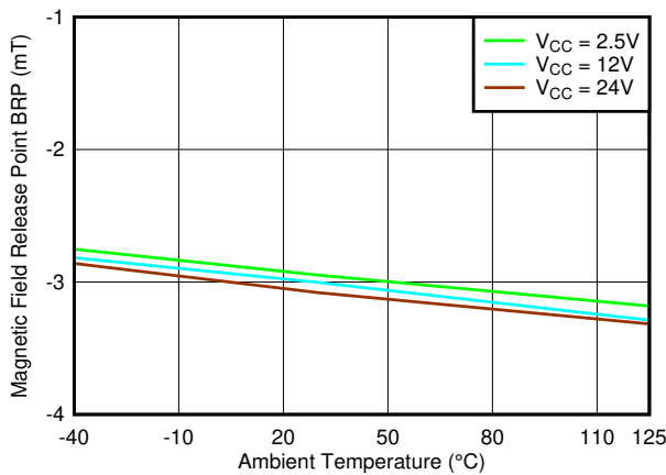
Figure 7-48. BRP_X Threshold vs. Temperature
