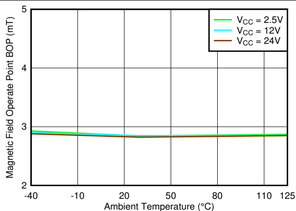
Figure 7-46. BOP_X Threshold vs. Temperature
