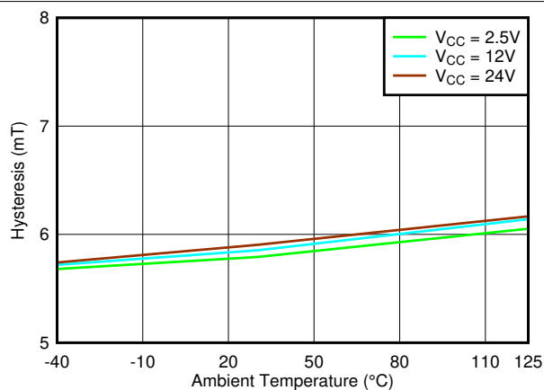
Figure 7-50. Hysteresis_X vs. Temperature
