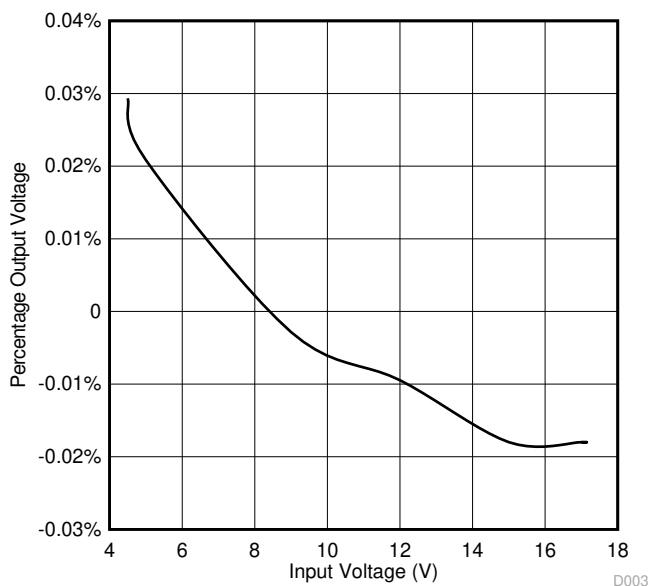
Figure 4-3. Line Regulation
