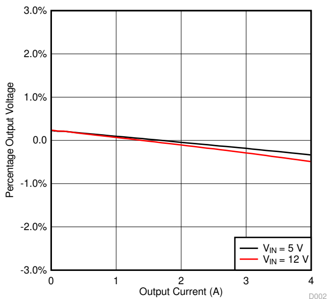
Figure 4-2. Load Regulation
