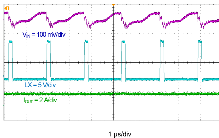
Figure 4-8. TPS564208 Input Voltage Ripple
