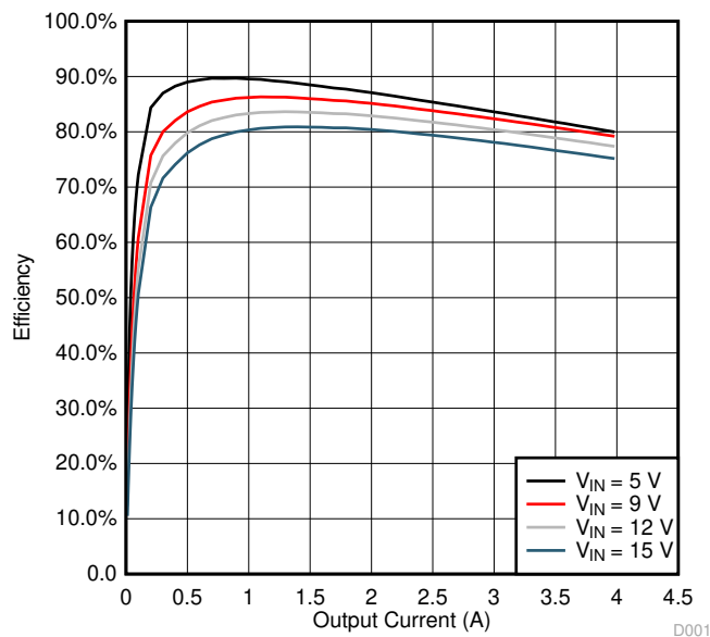
Figure 4-1. Efficiency
