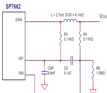
Fig. 21: Over Current Detection Circuit for I_{MAX} < (60\text{mV/DCR})
