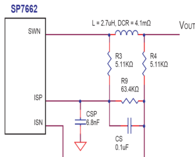
Fig. 20: Over Current Detection Circuit for I_{MAX} > 60\text{mV/DCR}
