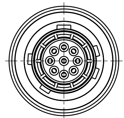
K10YCR-P09WCD0-0000 Mechanical coding: C Color coding: blue
