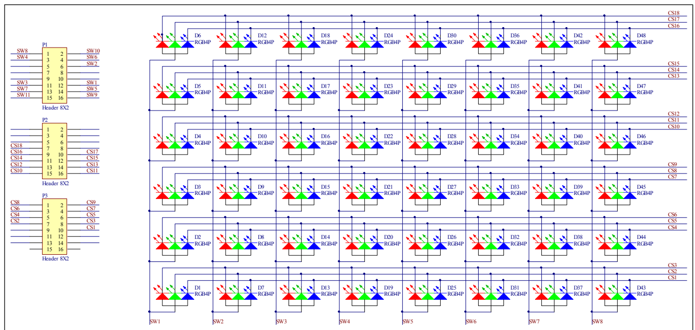
Figure 4: FxLED_6x8_ARRAY Schematic
