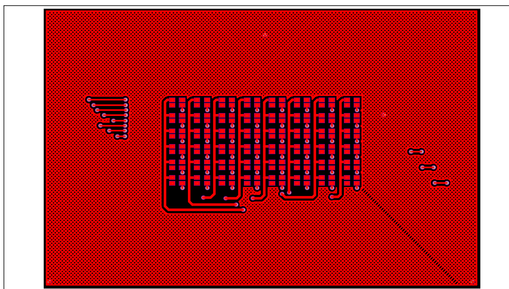
Figure 9: Board PCB Layout - Top Layer
