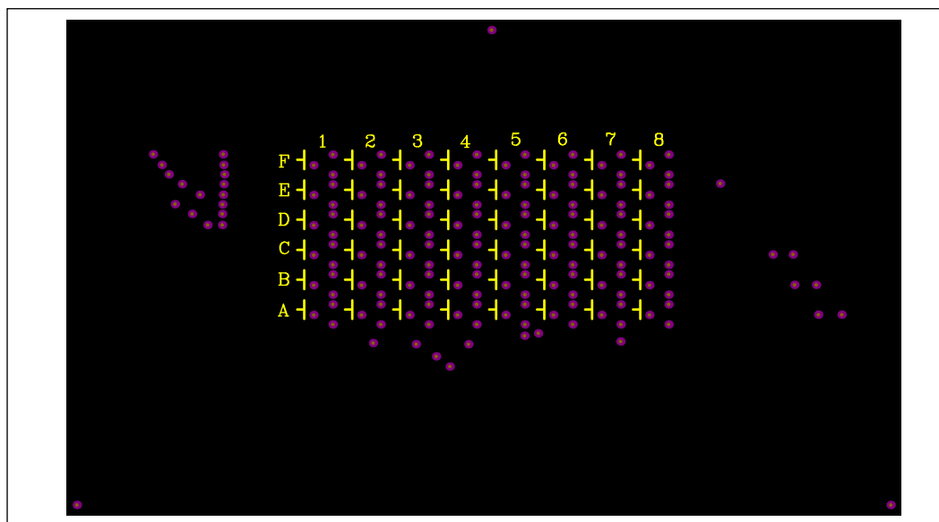
Figure 8: Board Component Placement Guide - Top Layer
