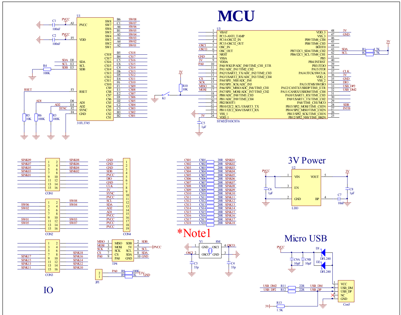
Figure 3: IS31FL3745 Application Schematic
