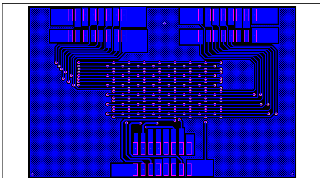
Figure 11: Board PCB Layout - Bottom Layer
