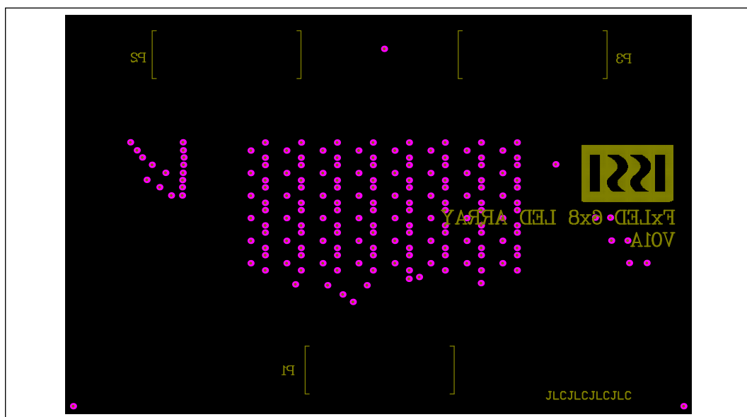
Figure 10: Board Component Placement Guide - Bottom Layer
