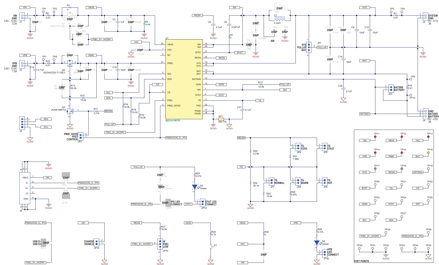
Figure 4-9. BQ25619EVM Schematic
