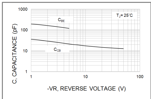
Fig.6 Typical Capacitance
