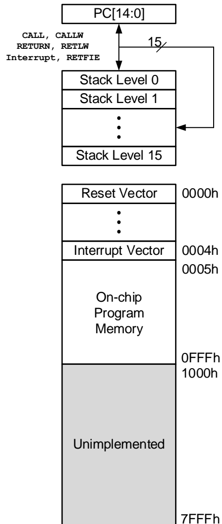
Figure 9-1. Program Memory and Stack (PIC16F180x4)
