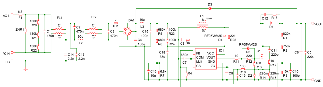
Figure 3. BD7693FJ-EVK-001 Schematics
