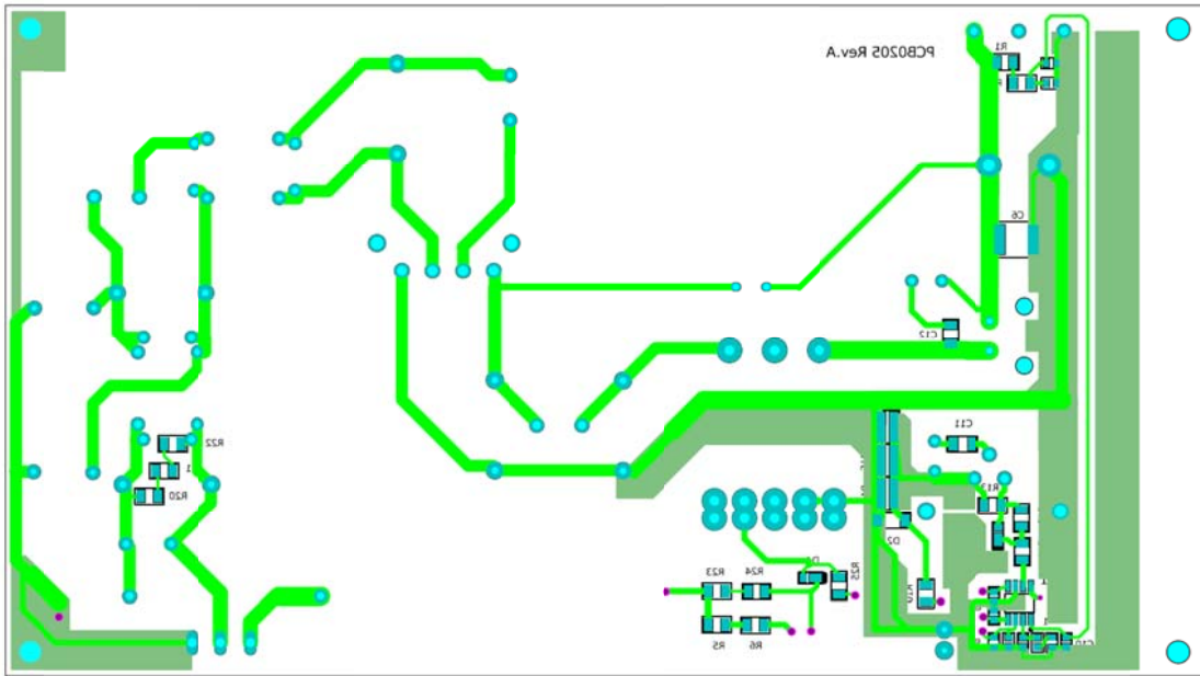
Figure 5. Bottom Layout (Top view)
