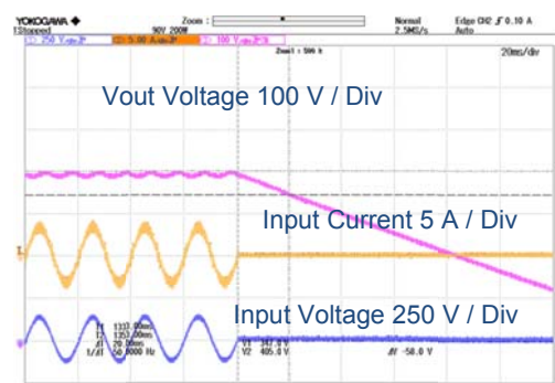
Figure 18. Hold time
