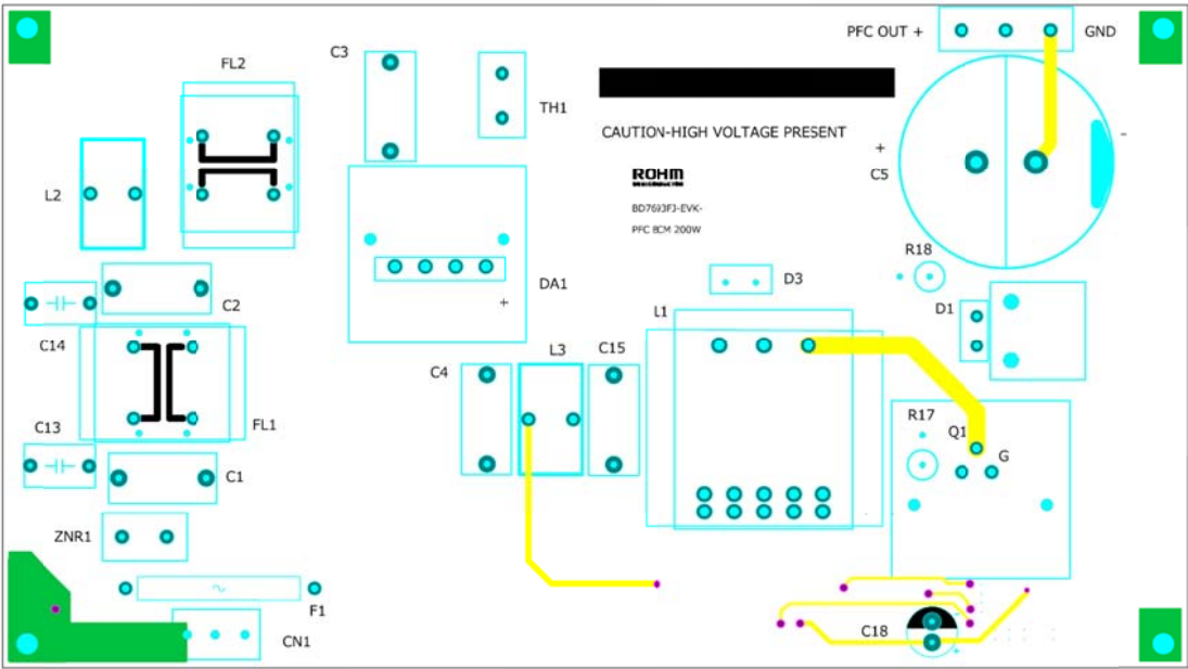
Figure 4. Top Silkscreen (Top view)
