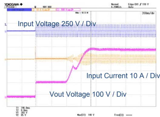
Figure 19. Start Up V_{IN} = 90\text{ V}_{ac}
