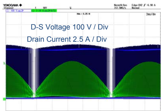
Figure 16. V_{DS}, I_D V_{IN} = 90\text{ V}_{ac} I_{OUT} = 0.5\text{ A}
