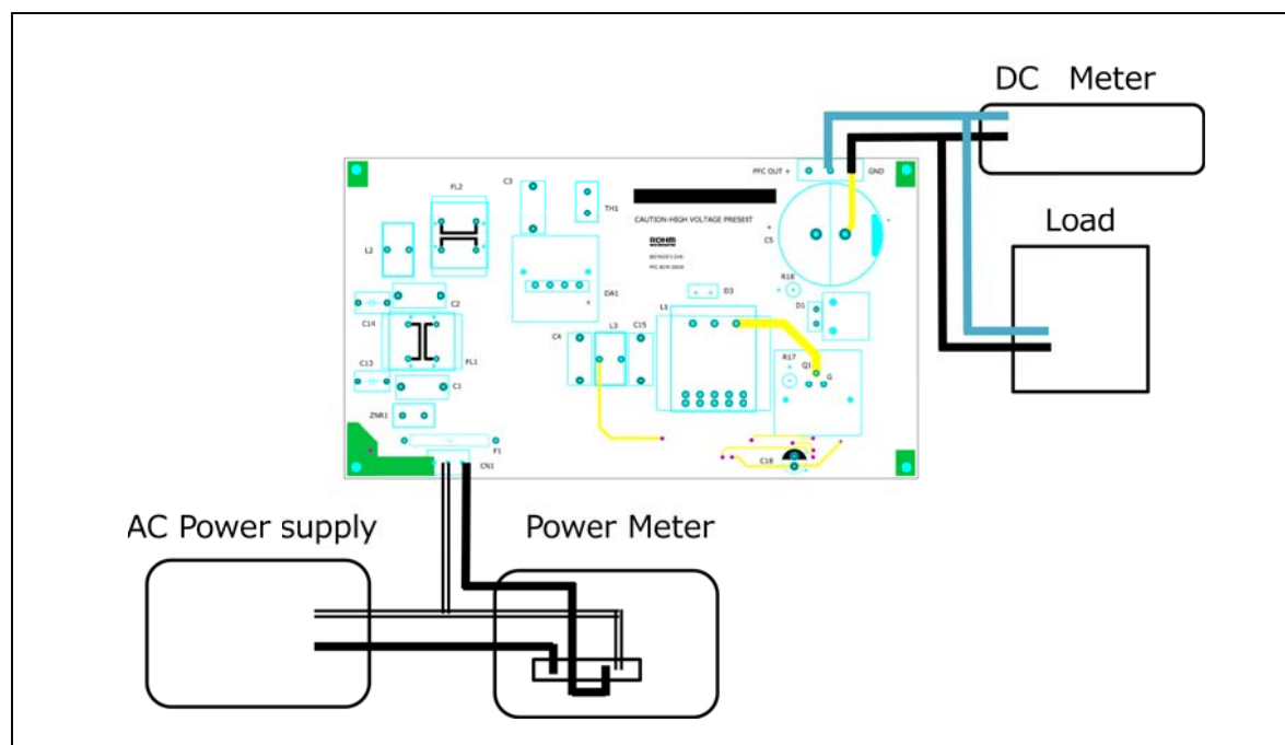
Figure 1. Connection Circuit
