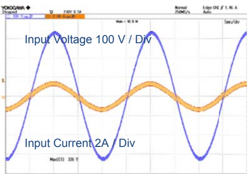
Figure 15. Input Current V_{IN} = 230\text{ V}_{ac} , I_{OUT} = 0.5\text{ A}
