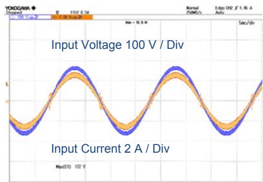
Figure 14. Input Current V_{IN} = 115\text{ V}_{ac} , I_{OUT} = 0.5\text{ A}
