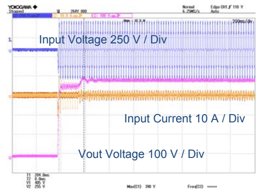
Figure 20. Start Up V_{IN} = 264\text{ V}_{ac}
