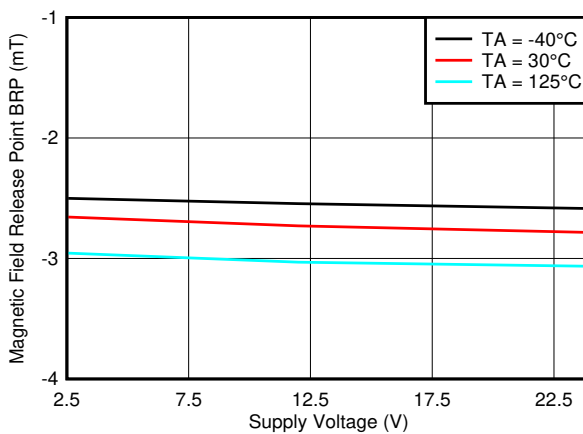
Figure 7-53. BRP_Y Threshold vs. V CC
