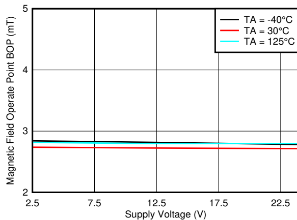
Figure 7-51. BOP_Y Threshold vs. V CC
