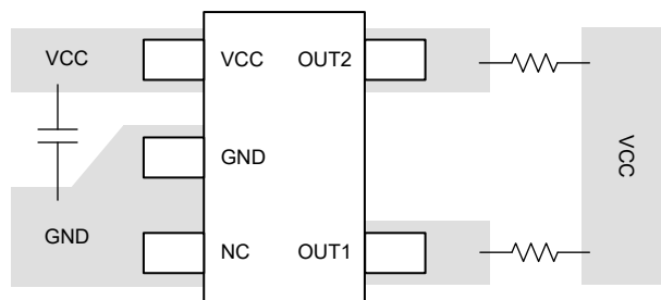
Figure 11-1. Layout Example
