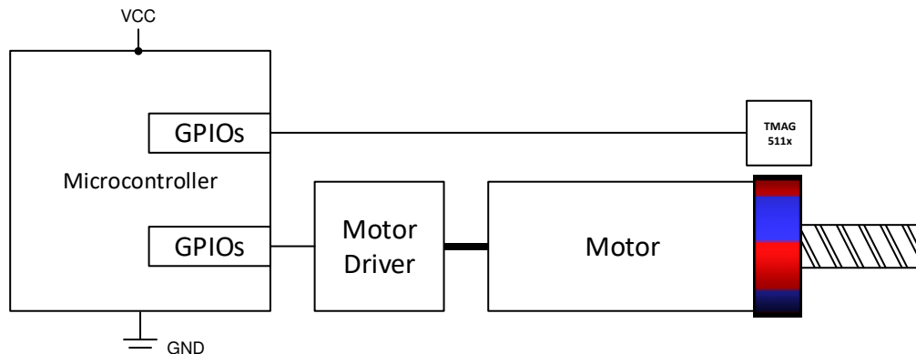
Figure 9-1. Incremental Encoding
