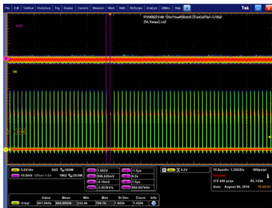
Figure 11-10. Output Ripple and SW Node of 1-V Output at 12 V IN , 25-A Output
