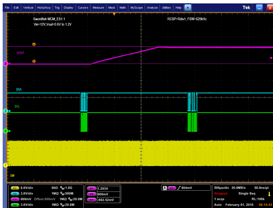
Figure 11-6. PMBus V OUT Step-Up = 0.6 V to 1.2 V at 25 A
