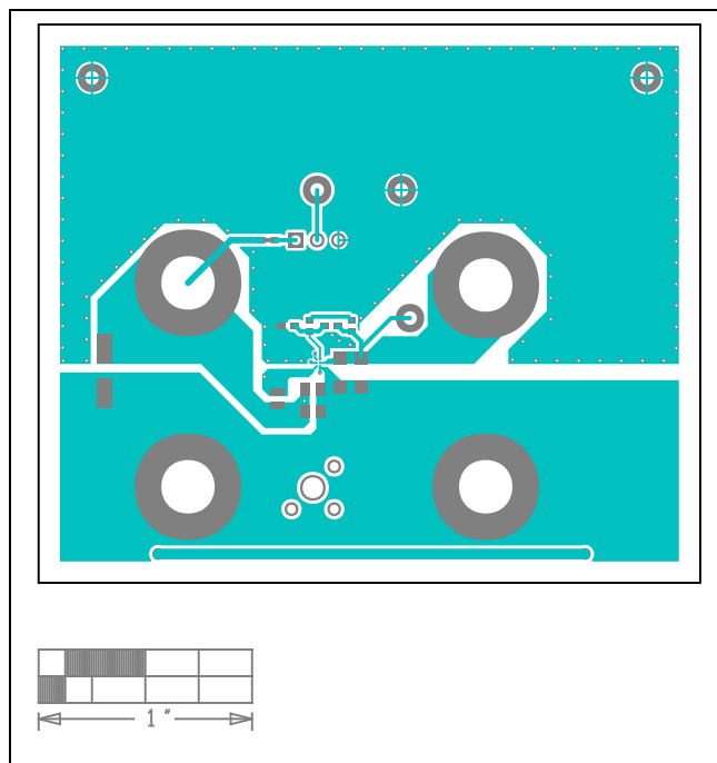
MAX17291B WLP EV Kit PCB Layout - Top
