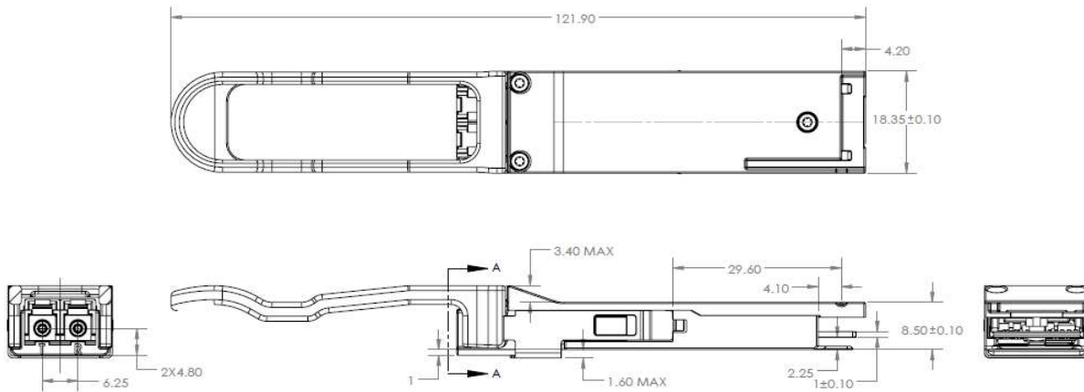
Figure 2 – FTL4C1QE3C mechanical drawing
