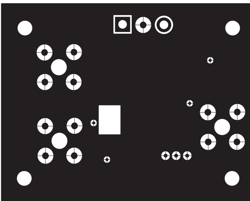
Figure 2–3. THS4031 EVM PC Board Layout – Back Side
