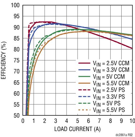
Figure 2. Measured Efficiency at f_{SW} = 2MHz
