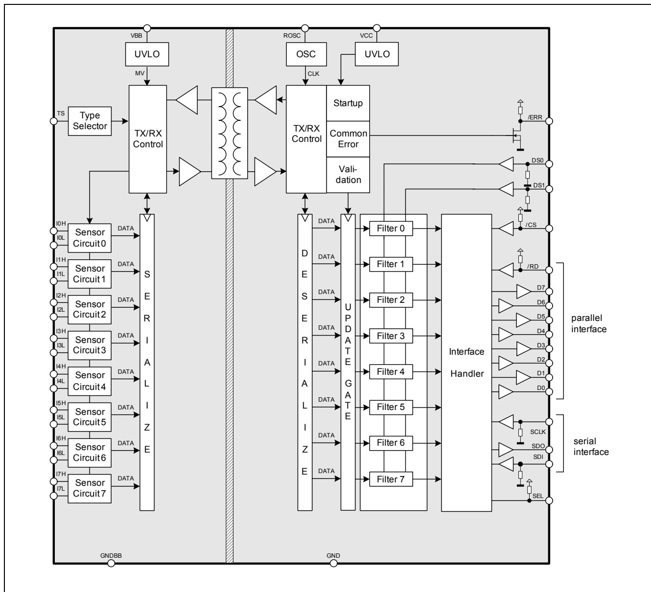
Figure 2 Block Diagram
