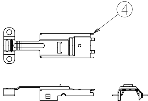
SHELL COVER
