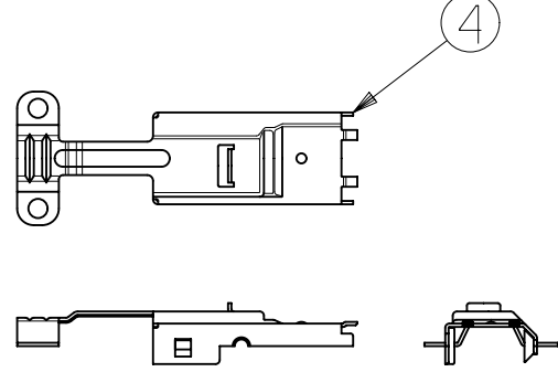
SHELL COVER
