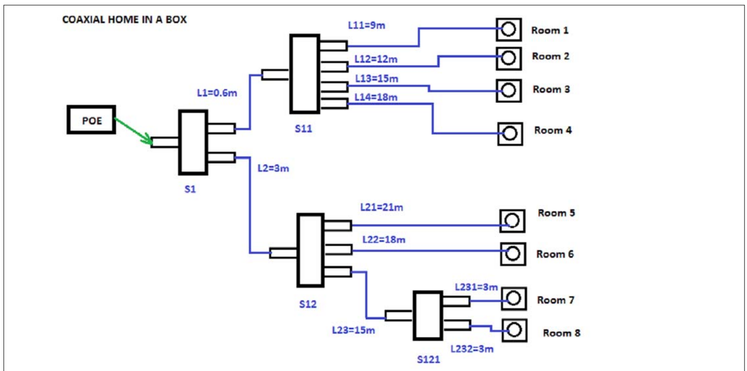
Figure 8: Coax "Home In A Box" Test Bench
