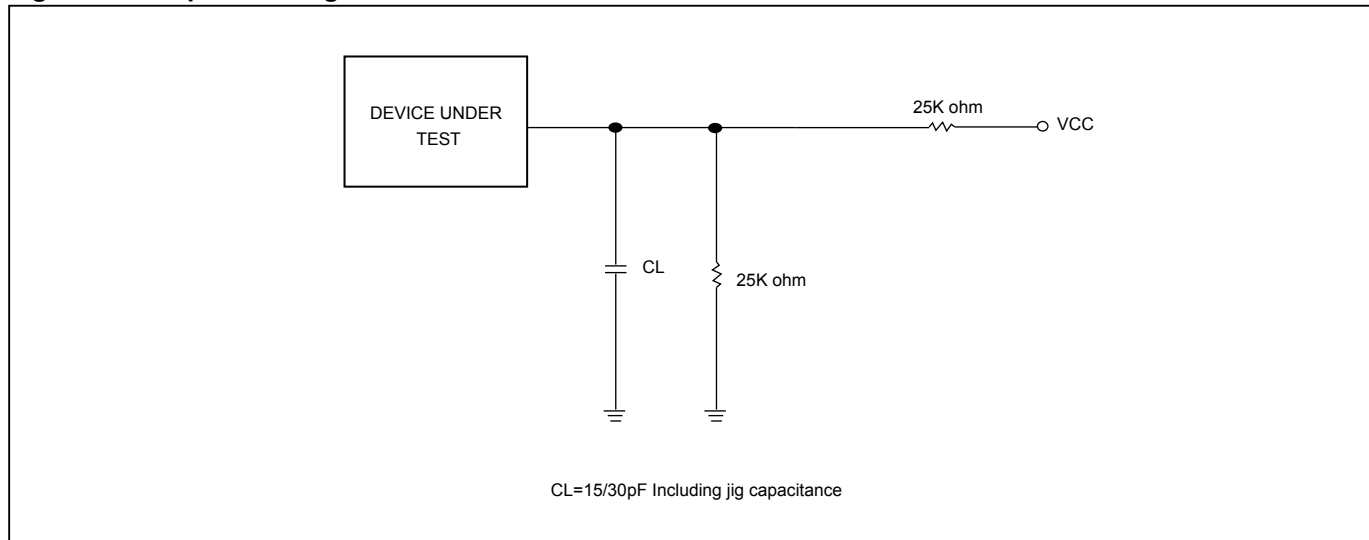
Figure 34. Output Loading
