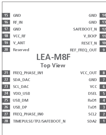
Figure 2: Pin Assignment
