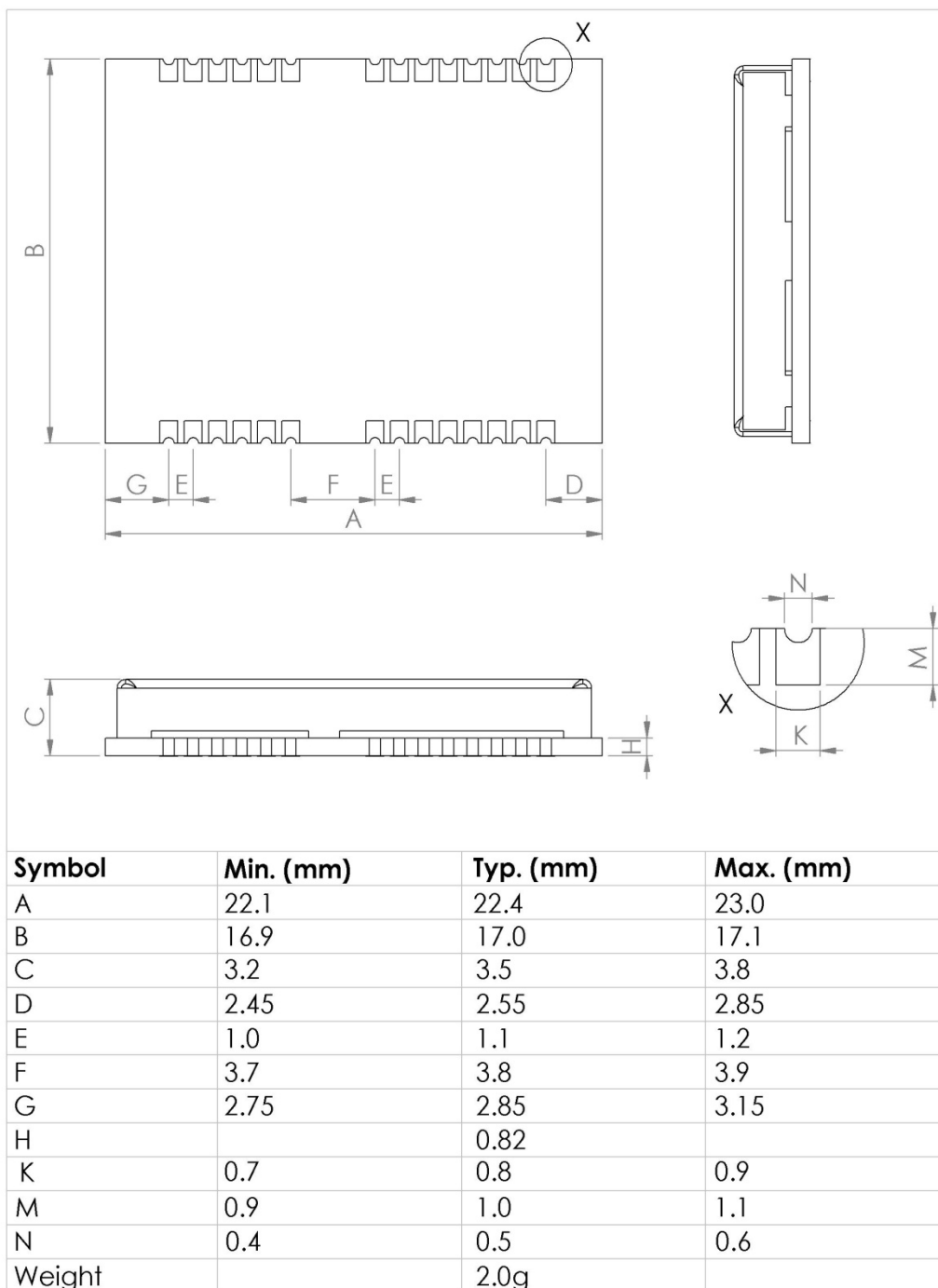
Figure 4: Dimensions
