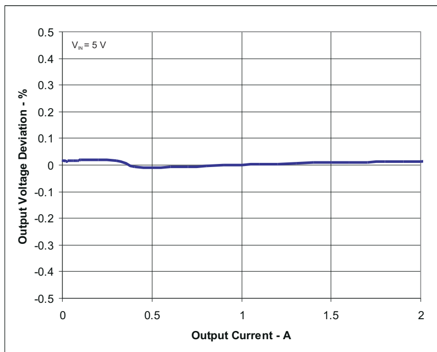
Figure 4-3. TPS54227EVM-686 Load Regulation, V_{IN} = 5\text{ V}
