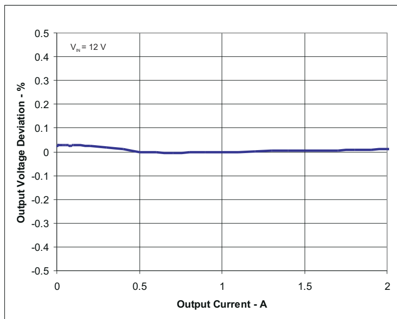
Figure 4-4. TPS54227EVM-686 Load Regulation, V_{IN} = 12\text{ V}
