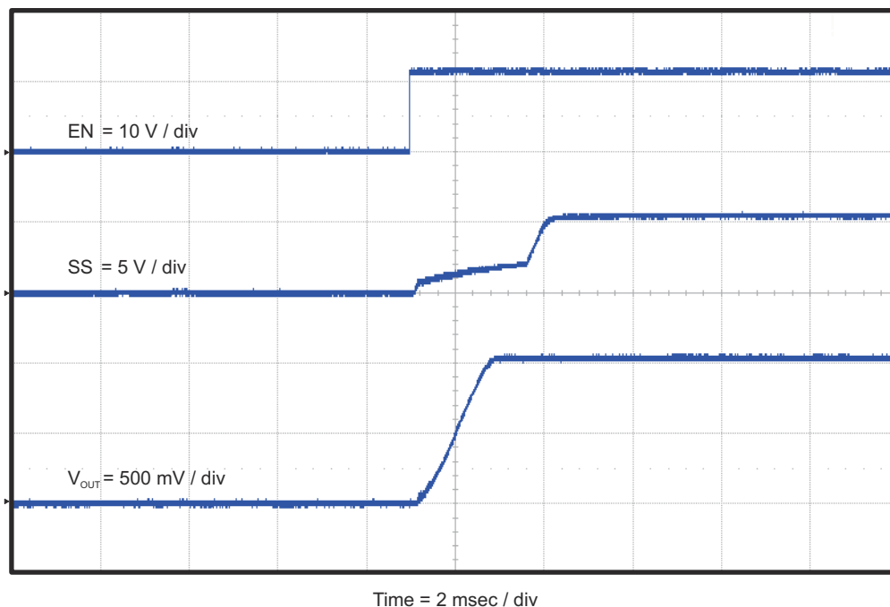
Figure 4-10. TPS54227EVM-686 Start-Up Relative to EN
