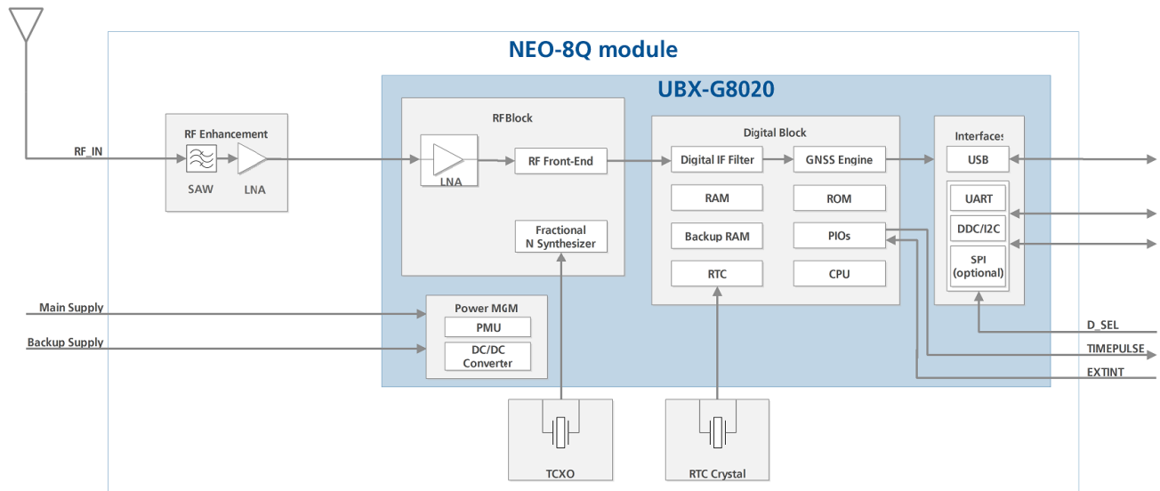
Figure 1: NEO-8Q block diagram
