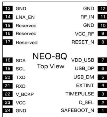
Figure 2: Pin assignment
