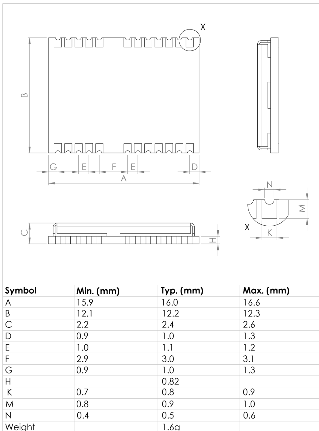
Figure 4: Dimensions
