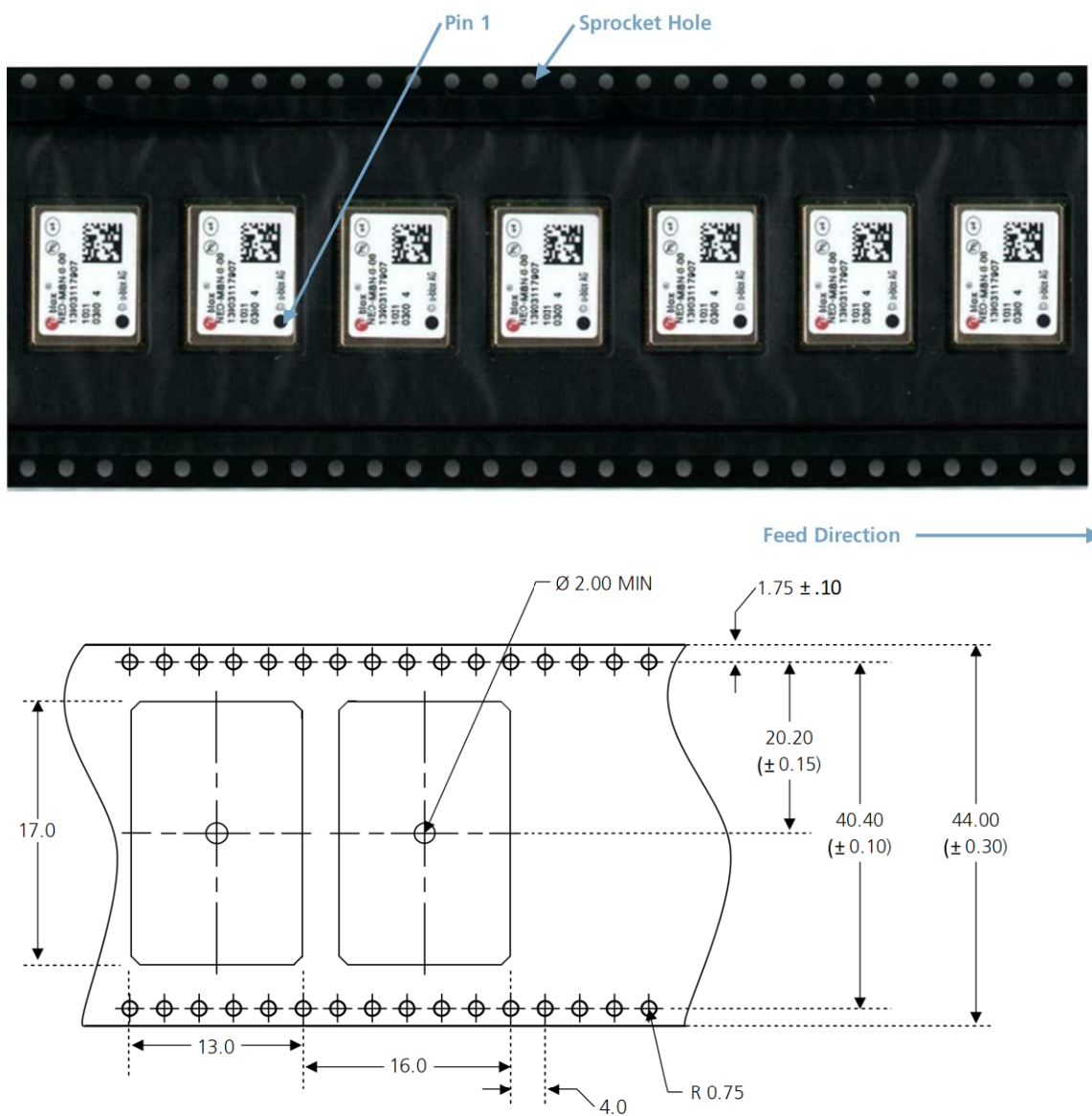
Figure 5: Dimensions and orientation for NEO-8Q modules on tape
