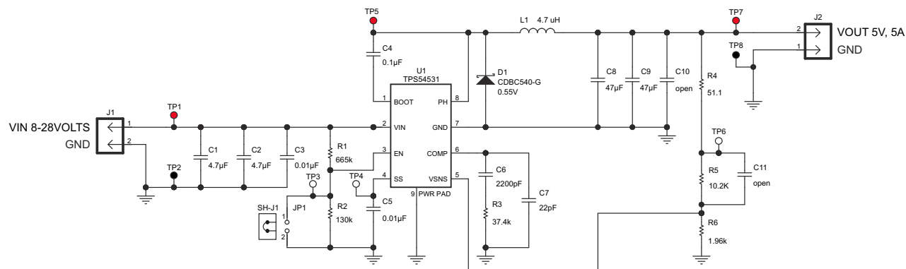
Figure 6-1. TPS54531EVM-530 Schematic Diagram
