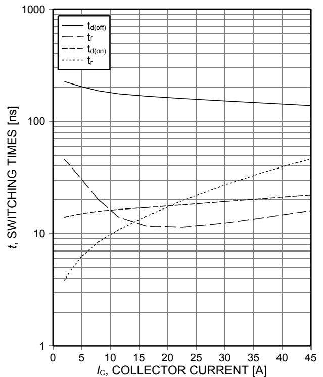
Figure 8. Typical switching times as a function of collector current (inductive load, T_j=150^{\circ}\text{C} , V_{CE}=400\text{V} , V_{GE}=15/0\text{V} , r_G=39\Omega , Dynamic test circuit in Figure E)
