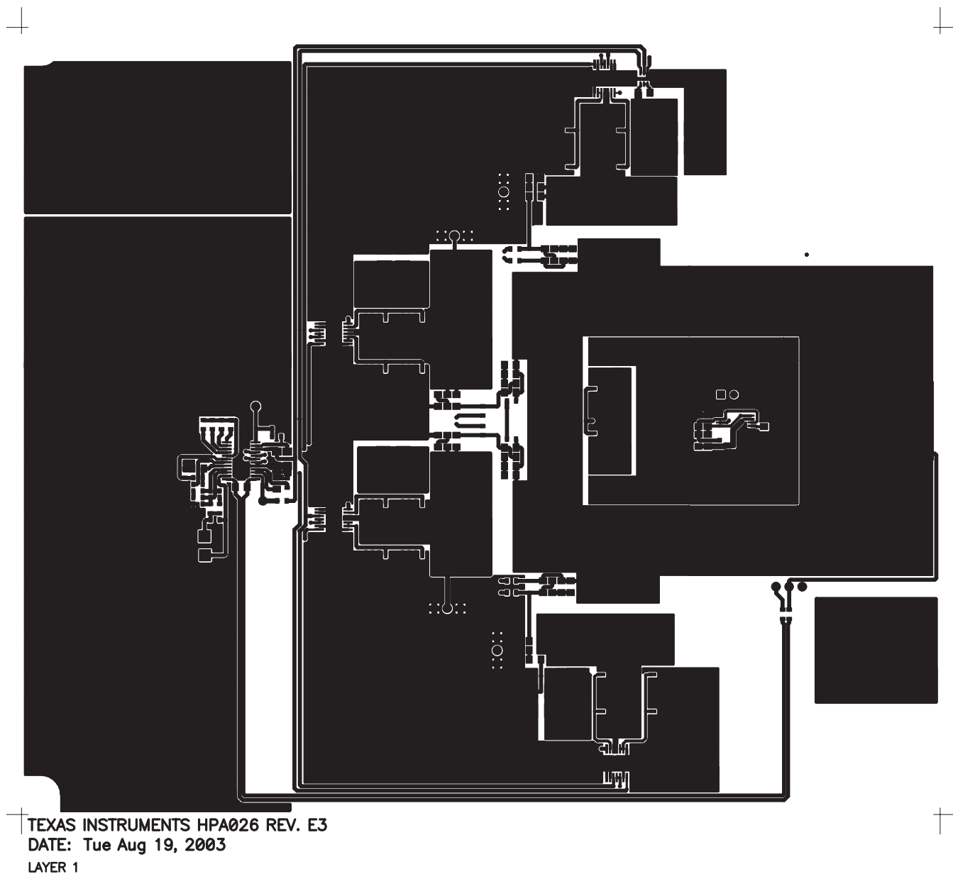
Figure 16. Top Side Copper
