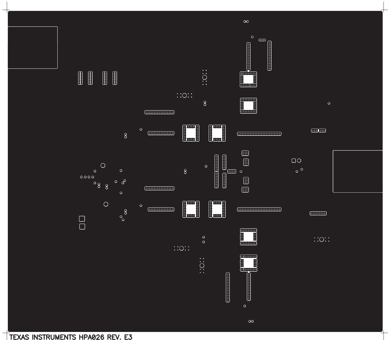
Figure 17. Internal 1 (Ground Plane)
