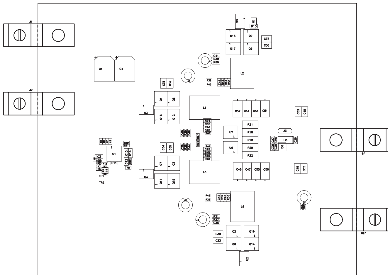
Figure 14. Top Side Component Assembly
