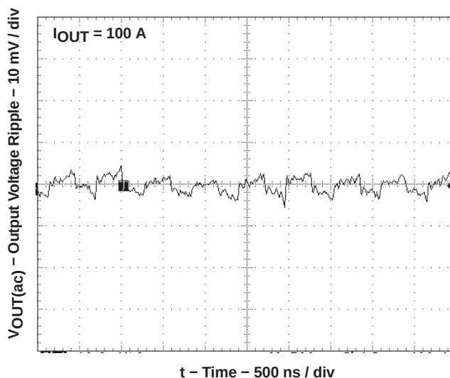
Figure 11. Output Noise
