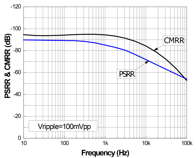
Figure 7. CMRR and PSRR vs. frequency
