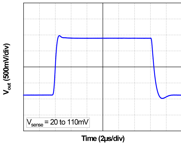
Figure 16. Step response for 20 to 110 mV V_{\text{sense}}
