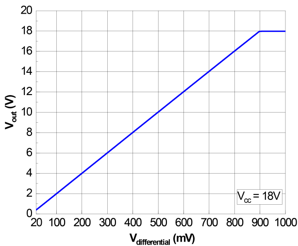
Figure 6. Gain plot
