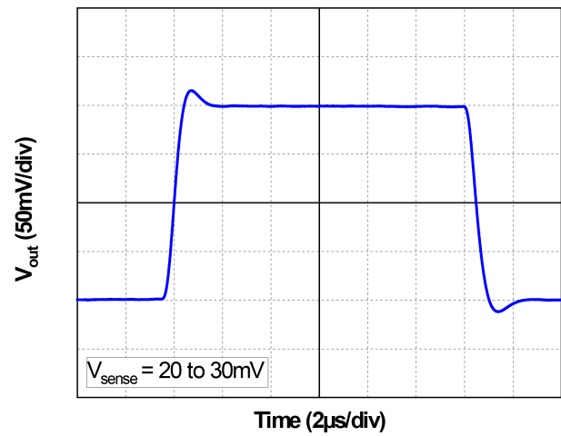
Figure 15. Step response for 20 to 30 mV V_{\text{sense}}
