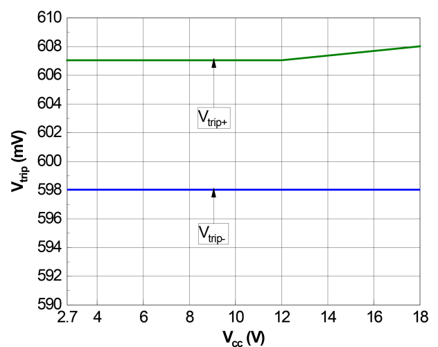
Figure 19. Comparator trip points vs. V_{\text{CC}}
