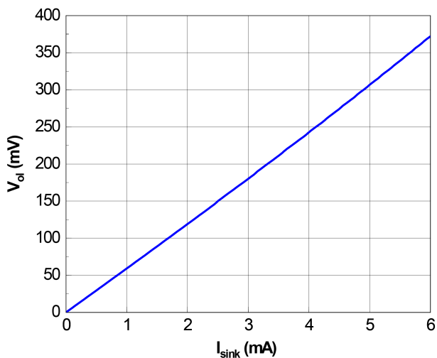
Figure 18. Comparator V_{\text{OL}} vs. I_{\text{SINK}}
