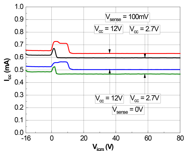
Figure 13. Quiescent current vs. common mode voltage
