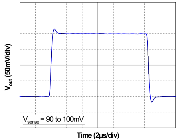
Figure 17. Step response for 90 to 100 mV V_{\text{sense}}
