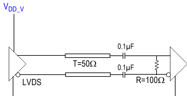
Figure 14. LVDS (STYLE = 0) AC Output Termination
