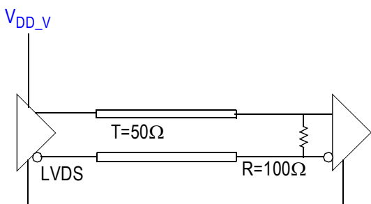
Figure 12. LVDS (STYLE=0) Output Termination
