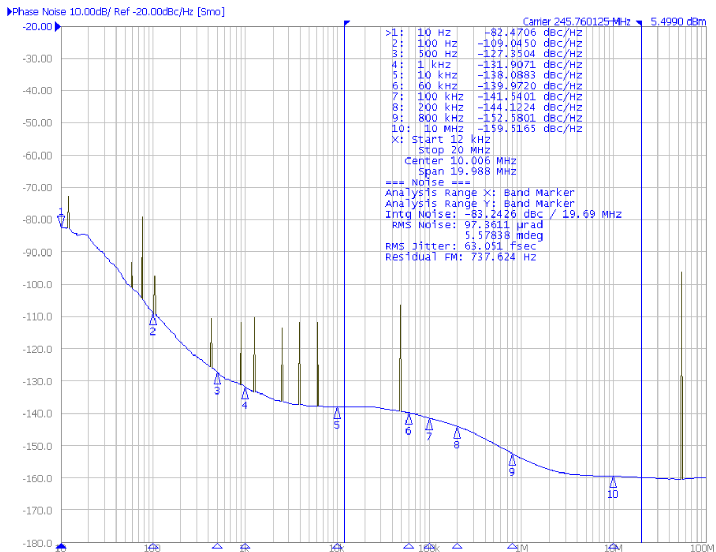
Figure 11. 245.76MHz Output Phase Noise
