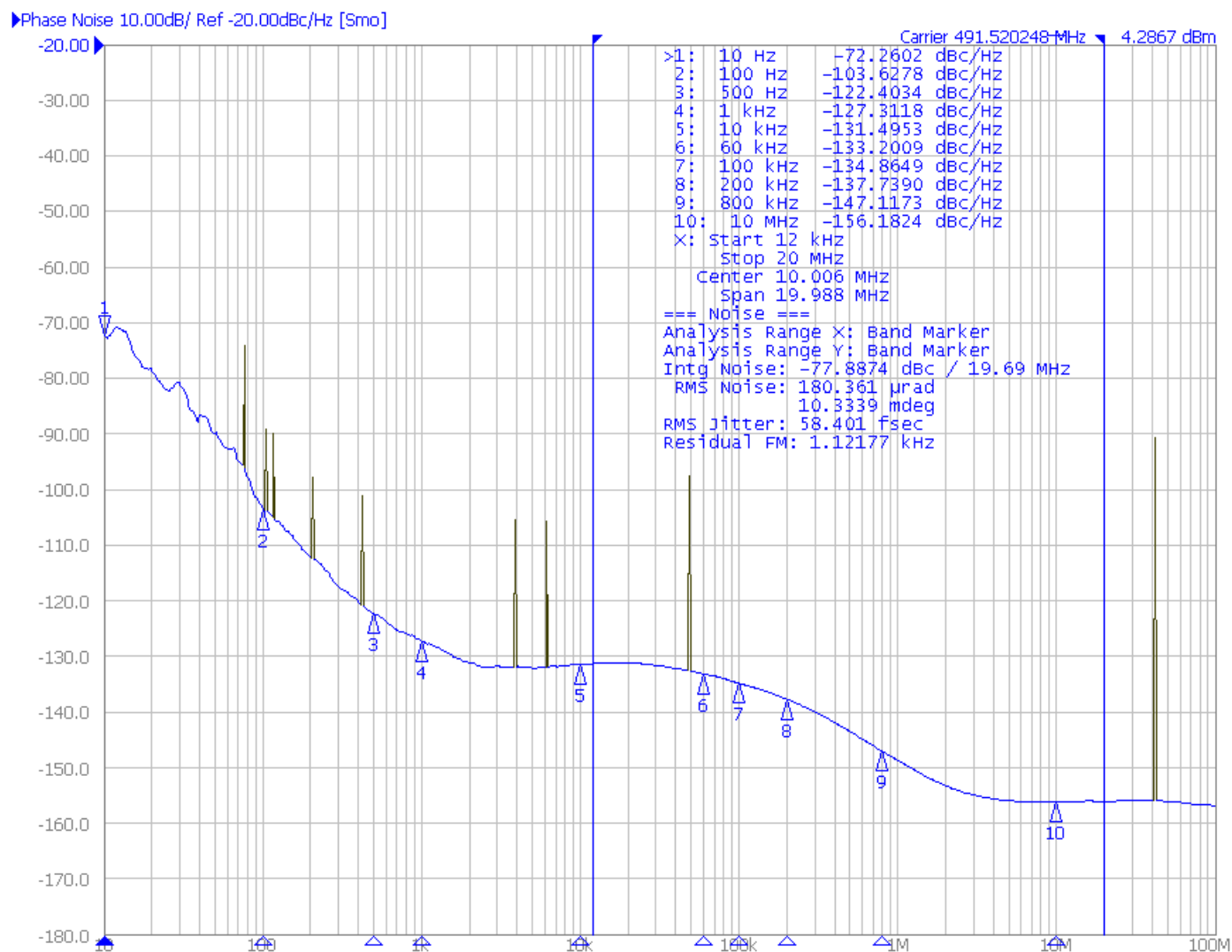
Figure 10. 491.52MHz Output Phase Noise
