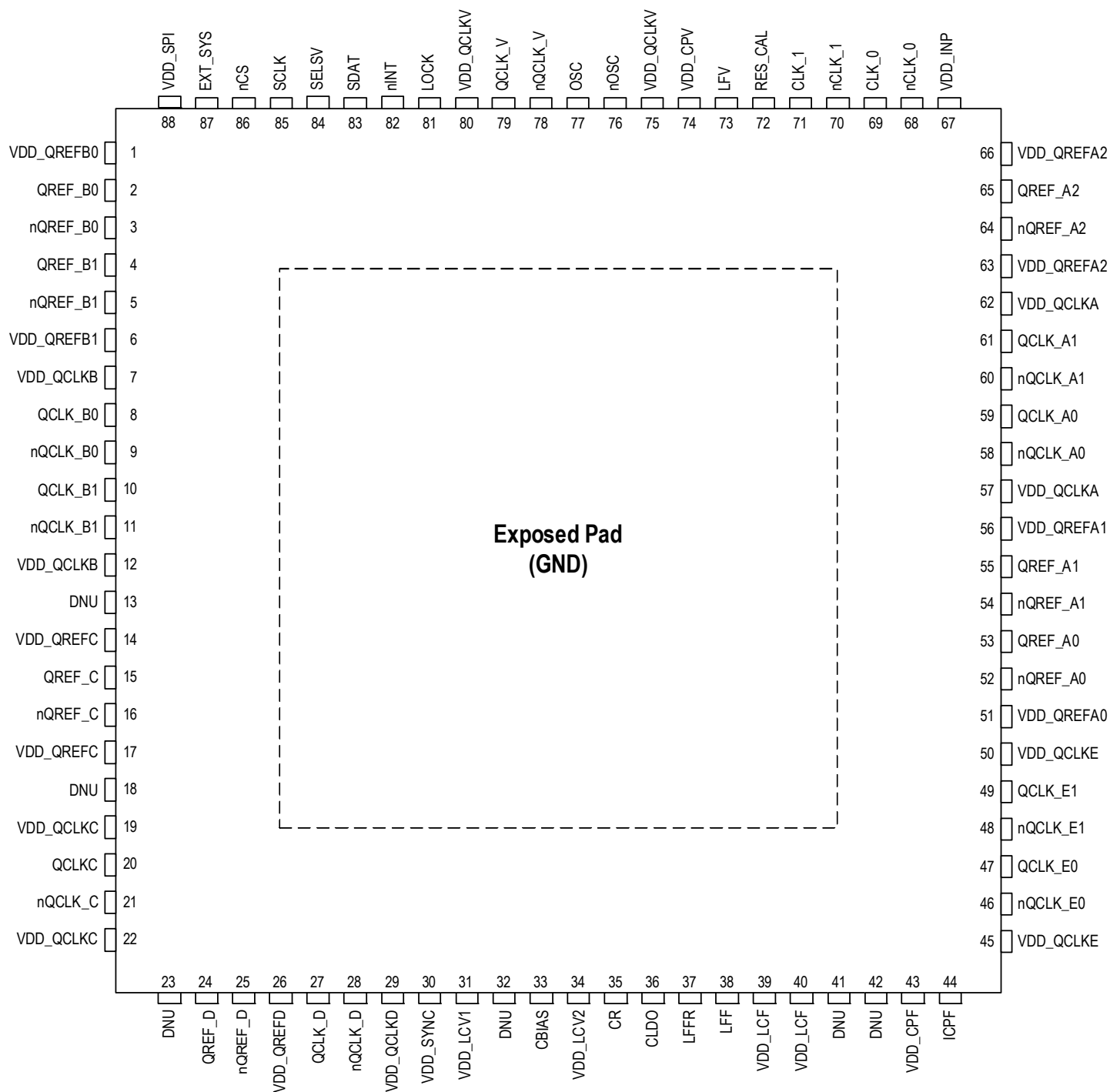
Figure 2. Pinout for 10 x 10 mm, 88-VFQFPN Package with Exposed Pad (Top View)
