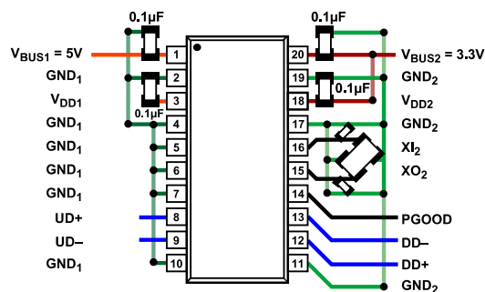
Figure 21. Required External Components and Connections (ADuM3166 with 5 V Supply to Side 1 and 3.3 V Supply to Side 2)
