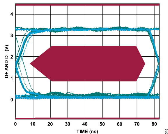
Figure 10. Full Speed Eye Diagram (Downstream Shown)
