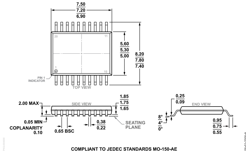
Figure 23. 20-Lead Shrink Small Outline Package [SSOP] (RS-20)
