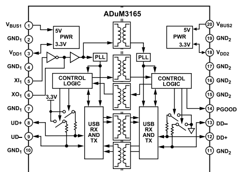
Figure 1. ADuM3165 (Clock Input from Host Side)
