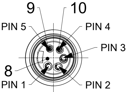
VIEW FROM THE FRONT SIDE
