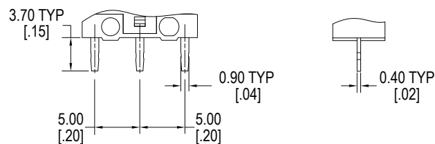
PC Pin
